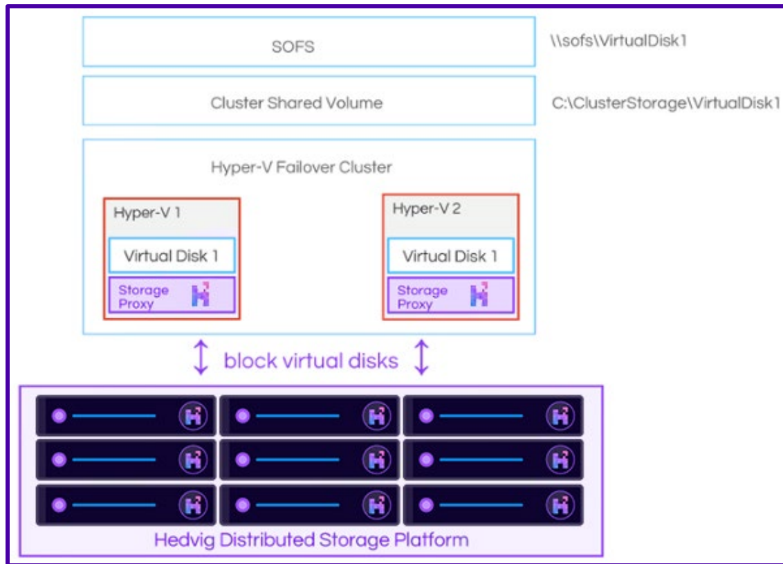
Figure 1: Hedvig + Hyper-V reference architecture
